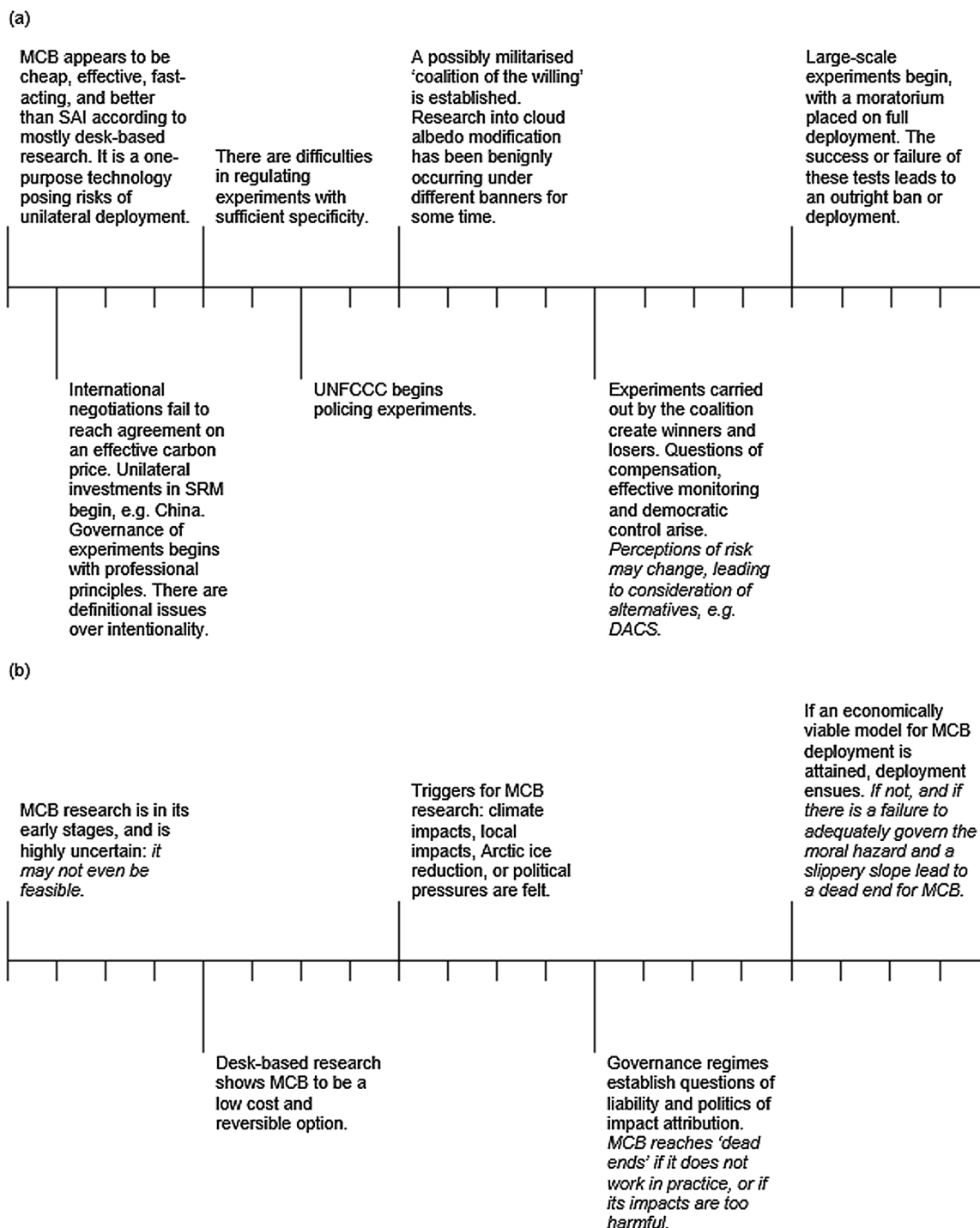
Fig. 4. Group 1 (panel a) and 2 (panel b) scenarios for marine cloud brightening. Time passes from left to right. Each marker along the timeline represents one year. Text in italics denotes possible scenario branching points.
